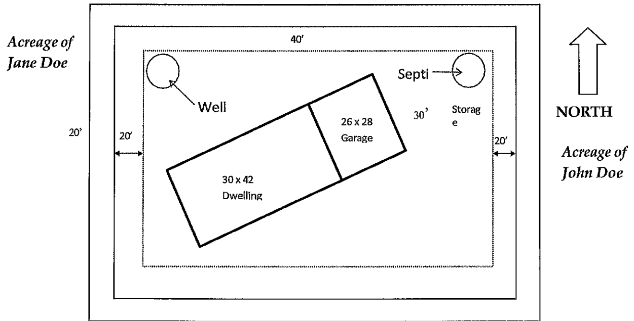
Figure III-2: Septic Design and Location
