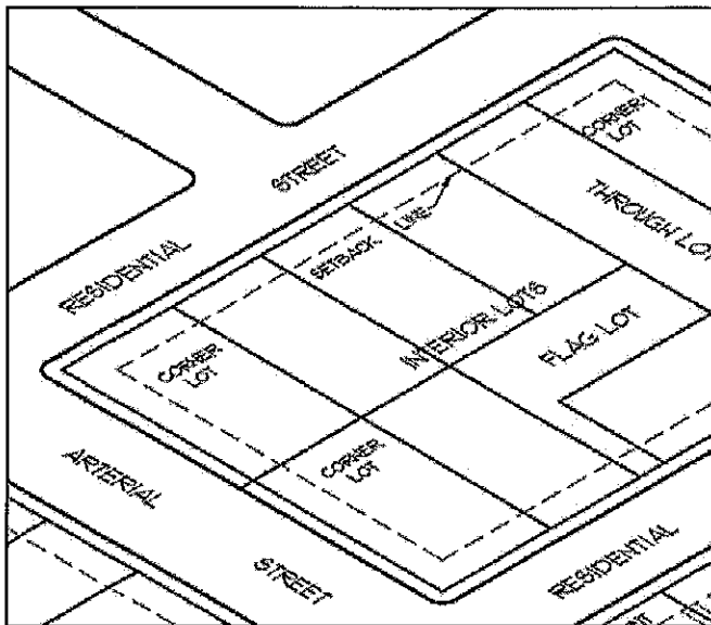
Figure III-1: Building Setback
